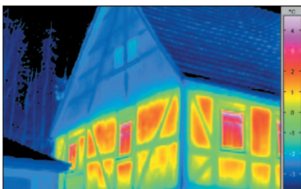
Half-timbered house
