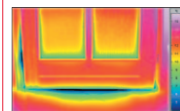
Detection of insulation problems (with Blower Door)
