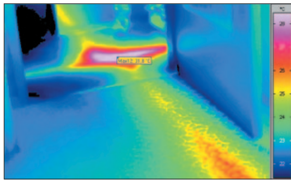
Leakage of a heating pipe
