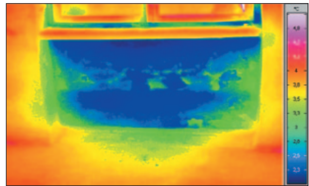
Humidity under a window
