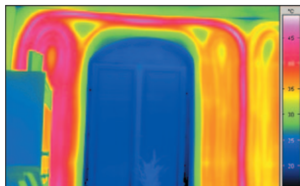
Wall heating system
