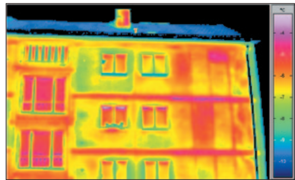
Building before renovation
