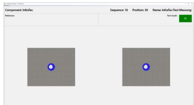
Fully automatic testing of resistance welding spots
