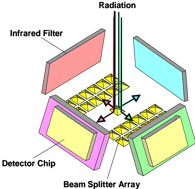
Fig. 1: Principle of reflective beamsplitting
